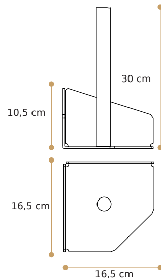
cod. 1707S
